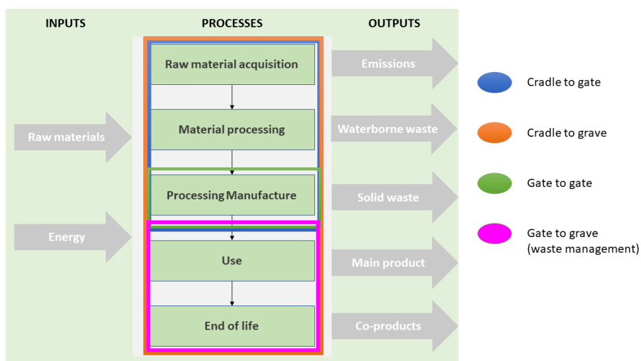
Figure 8: System boundaries (source: Authors)
