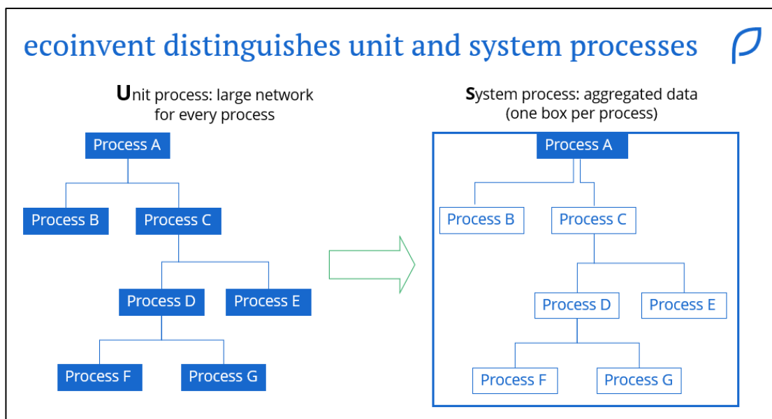
Figure 14: Difference between unit and system processes (Source: SimaPro Help Center 10 )
