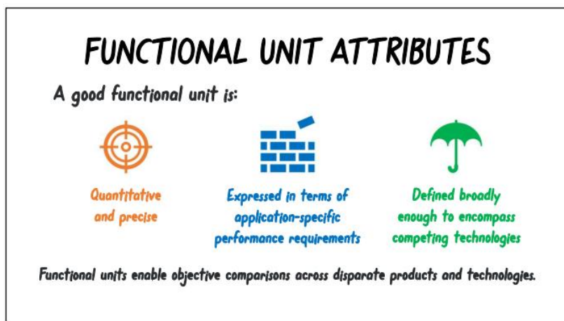
Figure 7: Key characteristics of a Functional Unit (Source: DOE (n.d))
