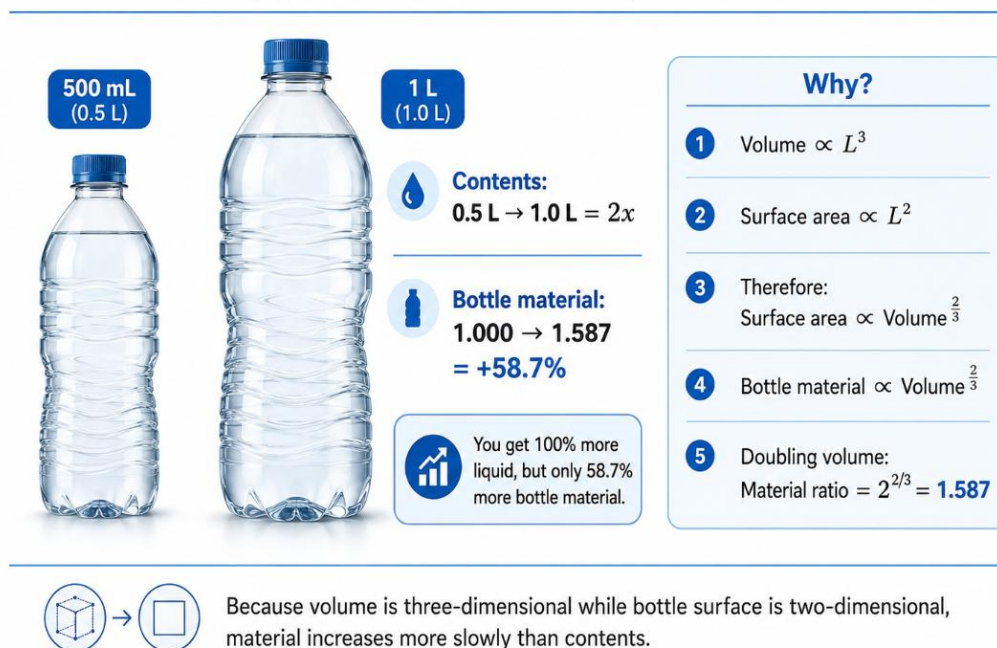
Figure 2: The surface area to volume ratio
